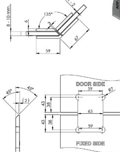
Glass cut option A: 45° fixed side
