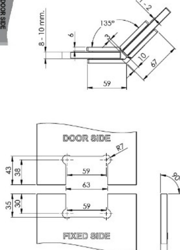
Glass cut option B: 90° fixed side
